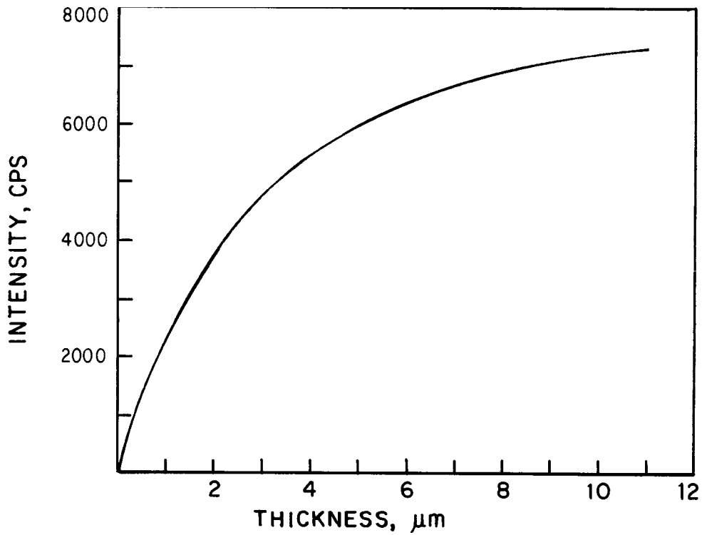
FIG. X1.1 Calibration Curve for the Determination of a Nickel Thickness by X-Ray Emission
