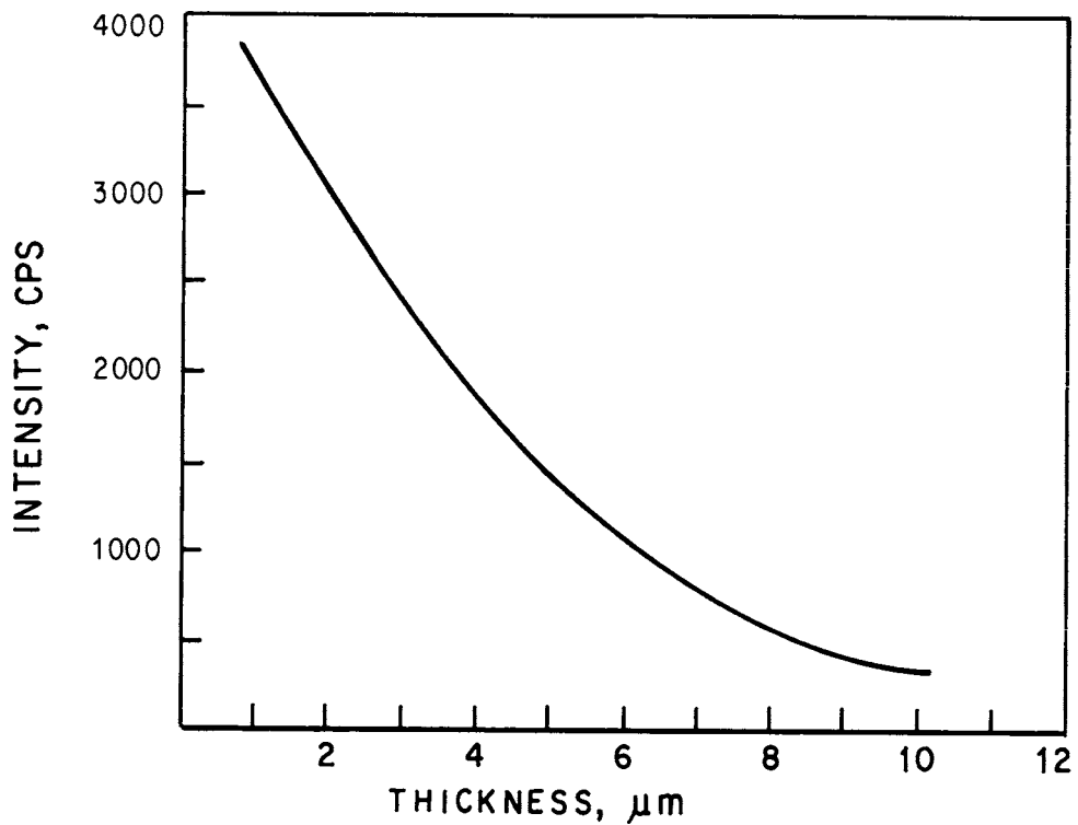
FIG. X1.2 Calibration Curve for the Determination of a Nickel Thickness by X-Ray Absorption
