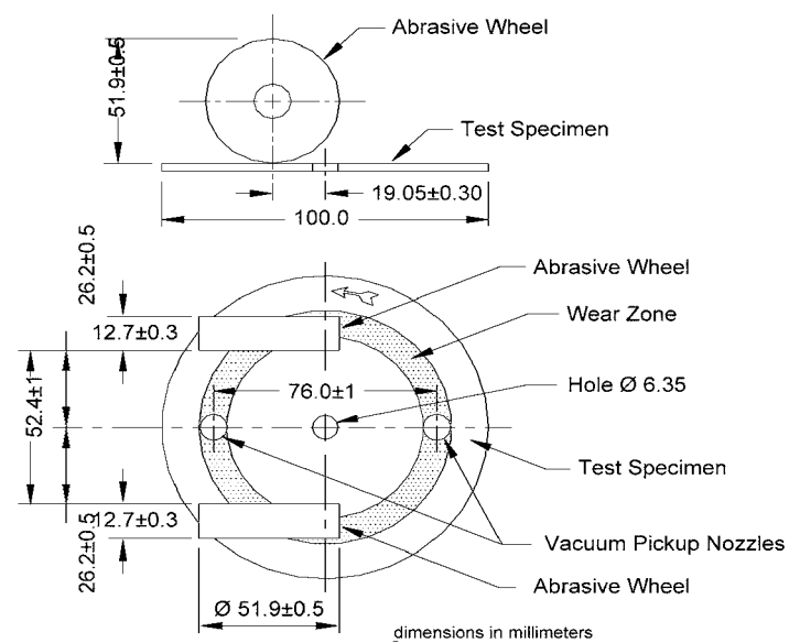
FIG. X1.1 Diagrammatic Arrangement of Taber Abraser Test Set-up
